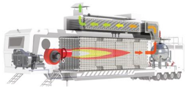
Figure N° 1. Portable Steam Generator of 50 MMBTU-Hr.
