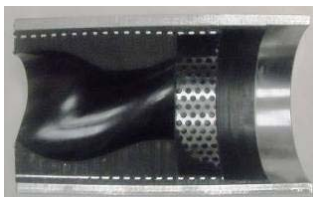
Fig. 7. Detail of reinforcement of chemical bonding by using stainless steel net welded to the stator tube.
