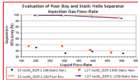
Fig. 2. Separation efficiency obtained in laboratory
